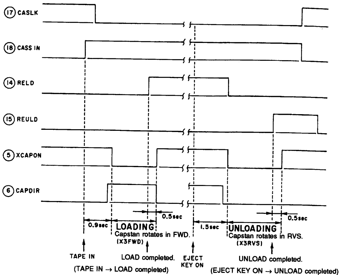
Figure 7-7. Load/Unload Timings
