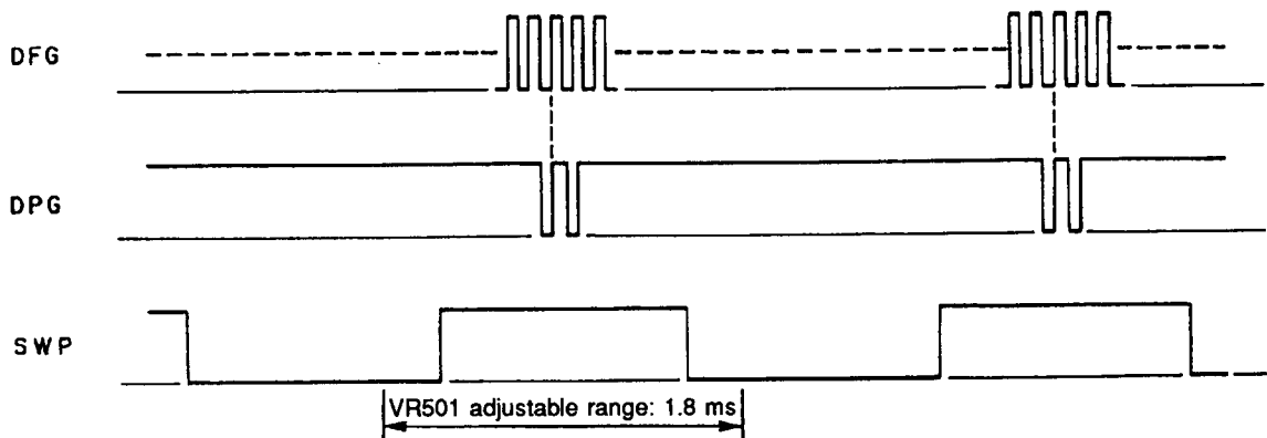
Figure 8-4. SWP Timing
