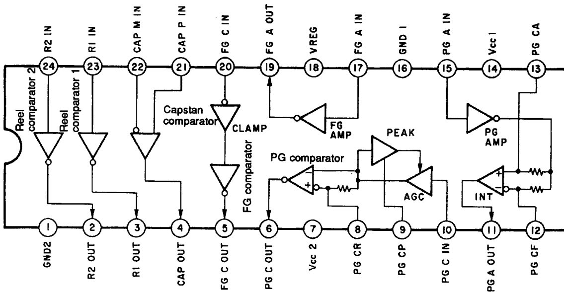
Figure 8-2. Block Diagram and Pin Assignment
