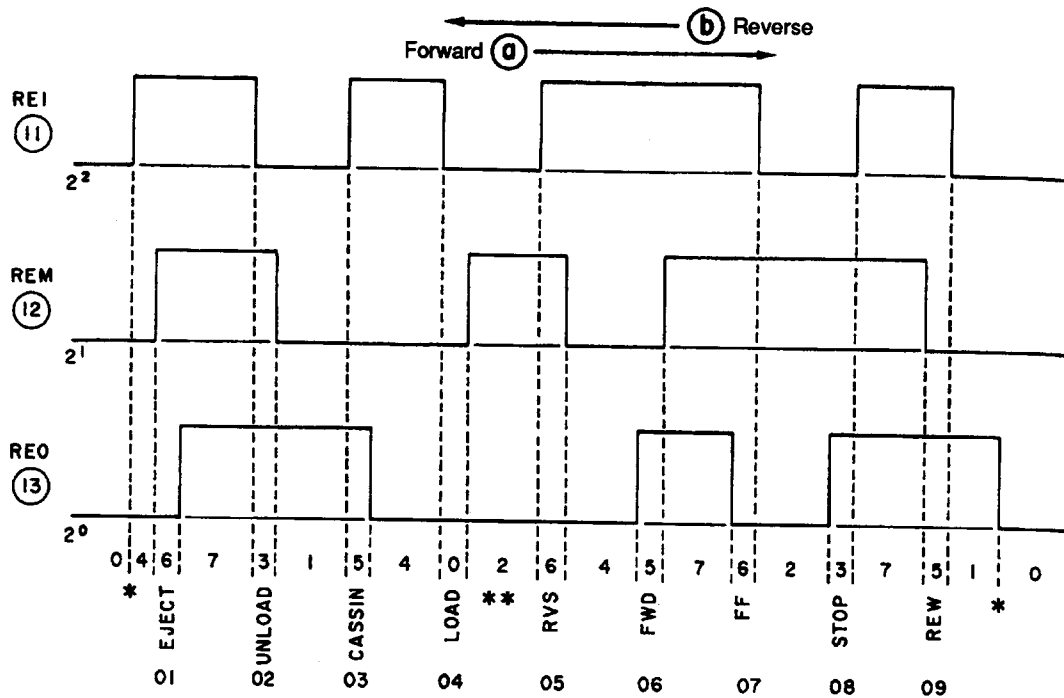
Figure 7-3. Rotary Encoder Pattern
